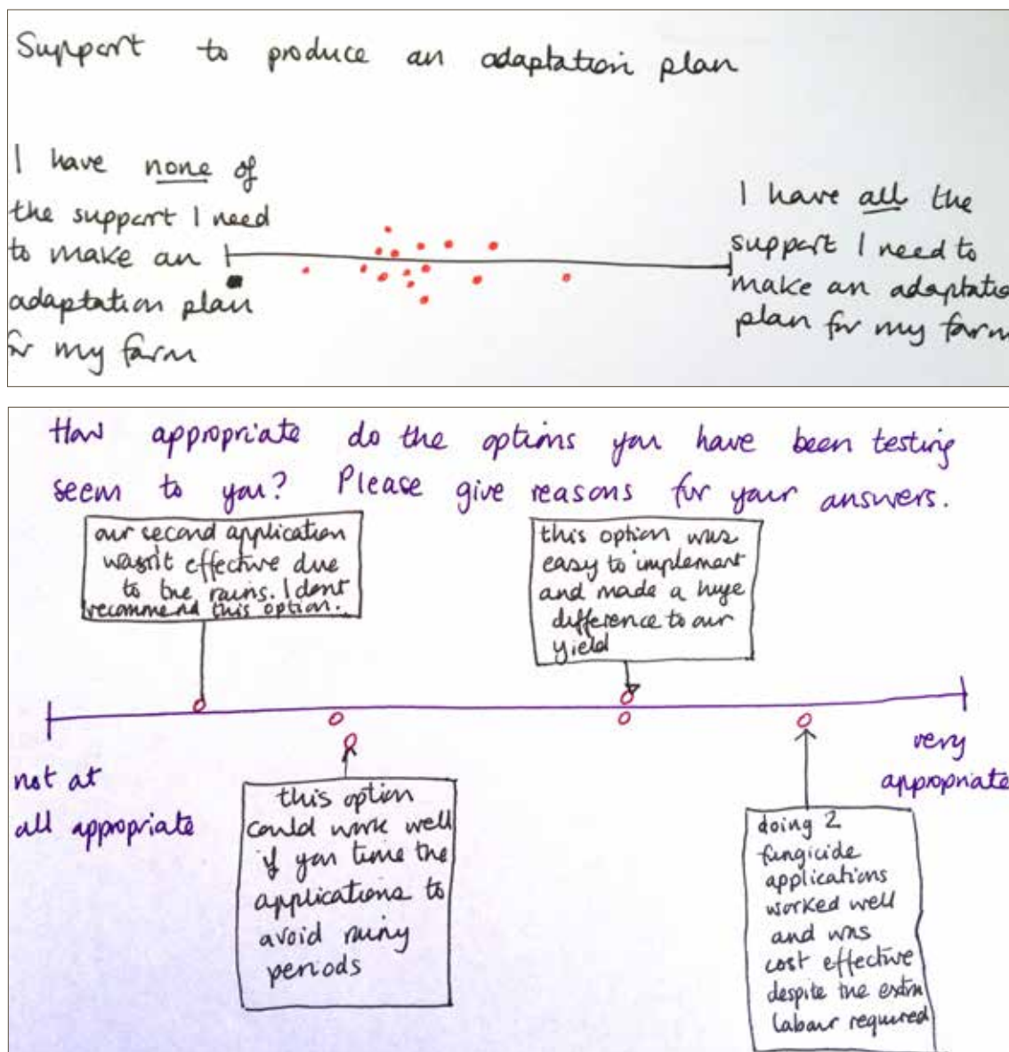
Figure 44: Spectrum lines
